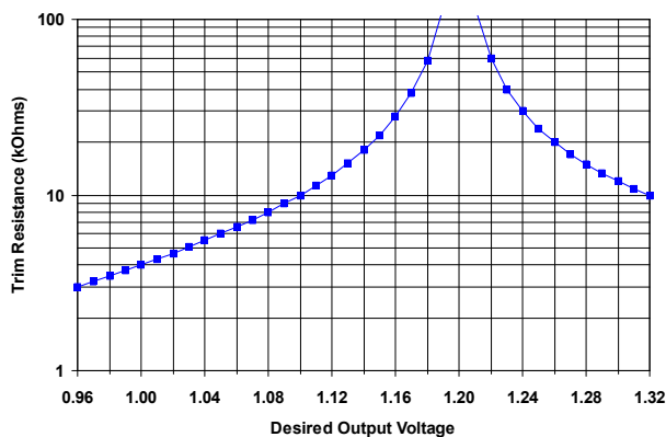
Figure C: Trim Graph for 1.2Vout module
